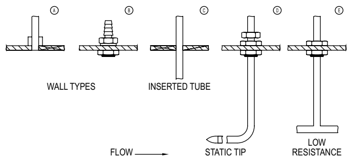
Figure 1 - Types of static pressure devices
