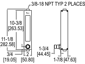
In-line meter
