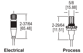
Probe connections
