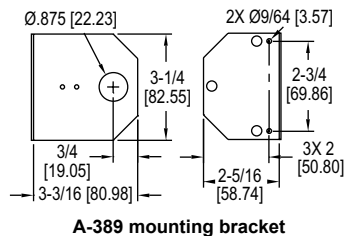
A-389 mounting bracket
