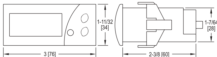
Panel cutout 2-51/64" x 1-9/64" (71 mm x 29 mm)
