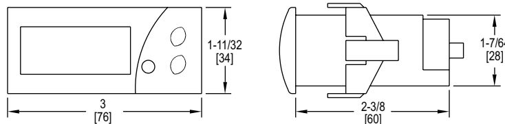
Panel cutout 2-51/64" x 1-9/64" (71 x 29 mm)
