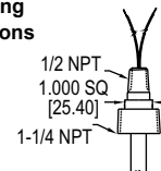
Type 2 mounting dimensions
