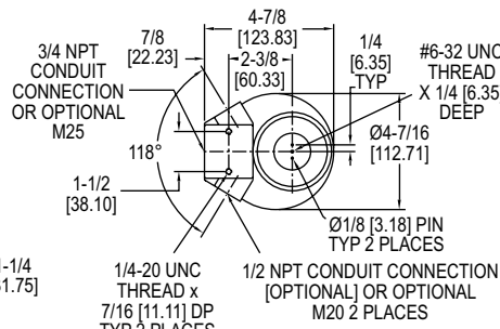
DIRECT DRIVE
