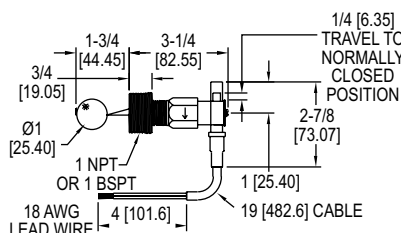
Spherical float
